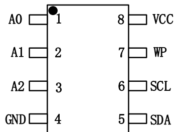
SOP-8L/TSSOP-8L/MSOP-8L (Top View)
