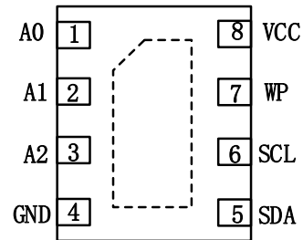
DFN-8L (Top View)
